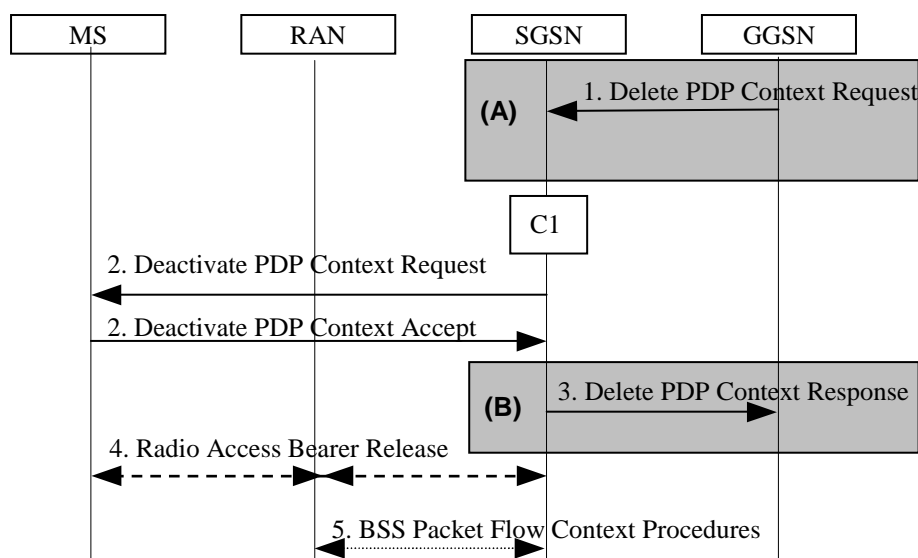
Figure 77: GGSN-initiated PDP Context Deactivation Procedure
