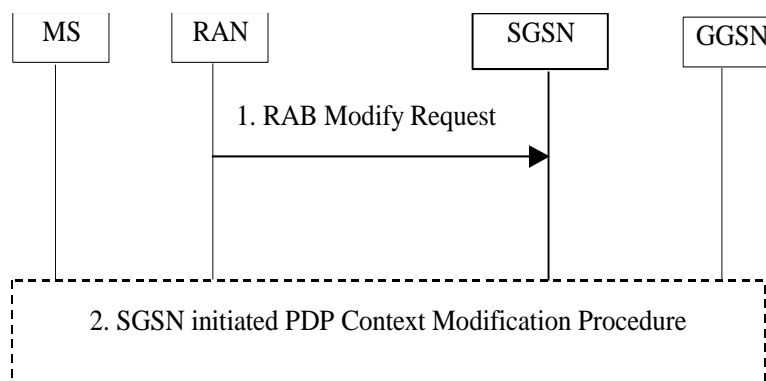
Figure 73: RAN-initiated RAB Modification Procedure
